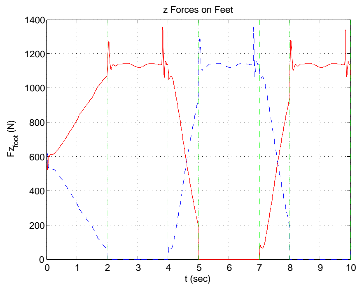
Figure 29. Step Machine: Vertical Forces on feet (dashed line = left leg).
